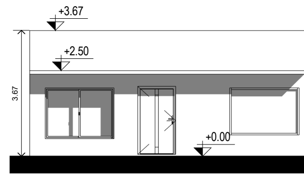
FACHADA PRINCIPAL
